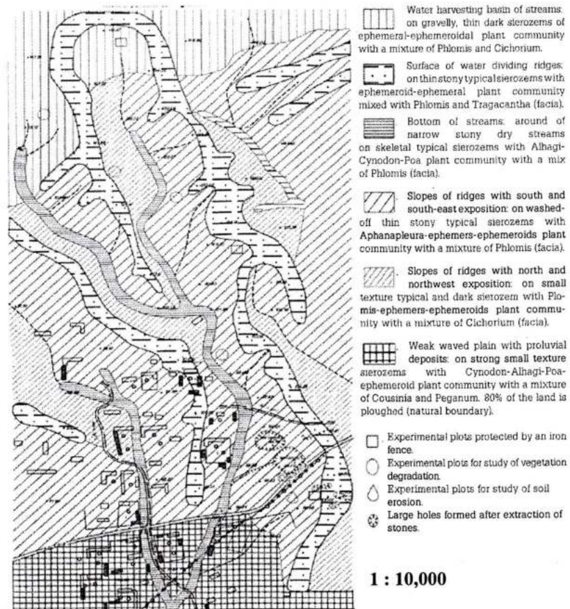
Fig. 1. Allocation of geosystems in Ishmantupsay basin in east part of Gobduntau mountain range.
